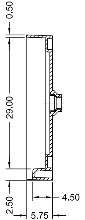
SECTION B-B
